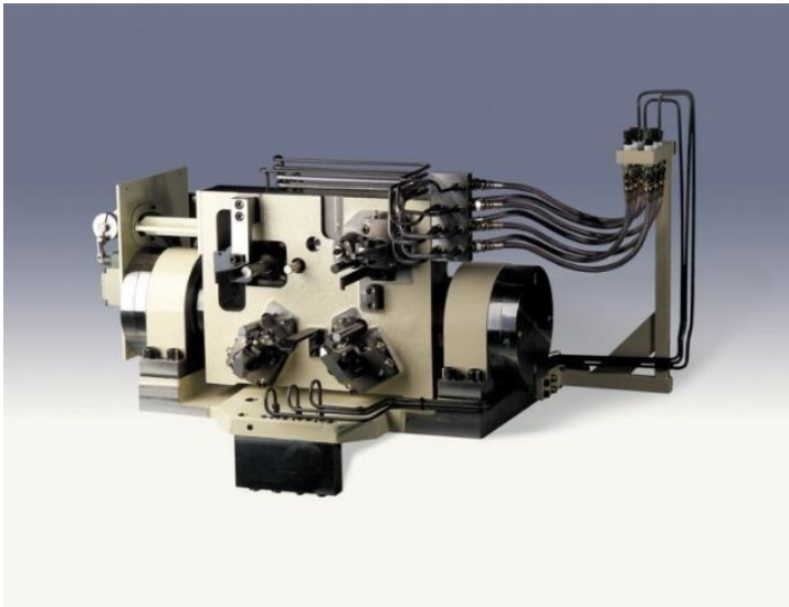
Tilting Jig for Workholding Fixture
