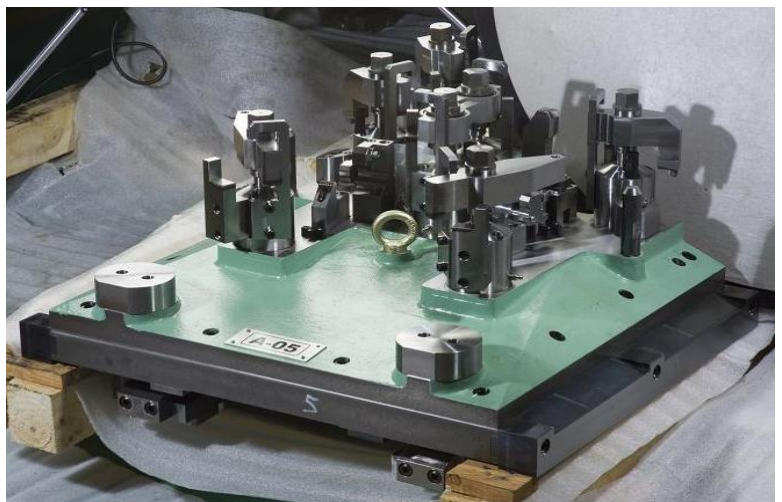
Jig for Steering Knuckle
