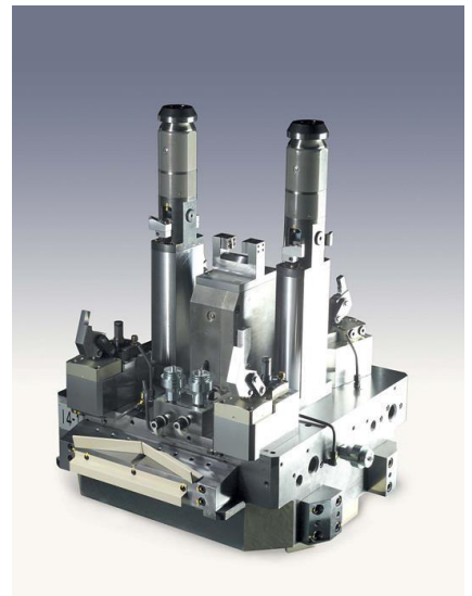
Engine Block Fixture
