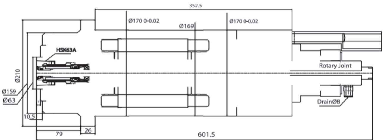
Technical drawing for SW170-2425-H63AECOT
