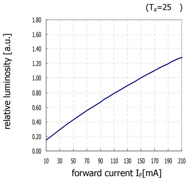
(2) forward current vs. relative luminosity
